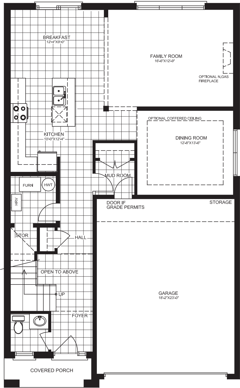
Ground Floor
